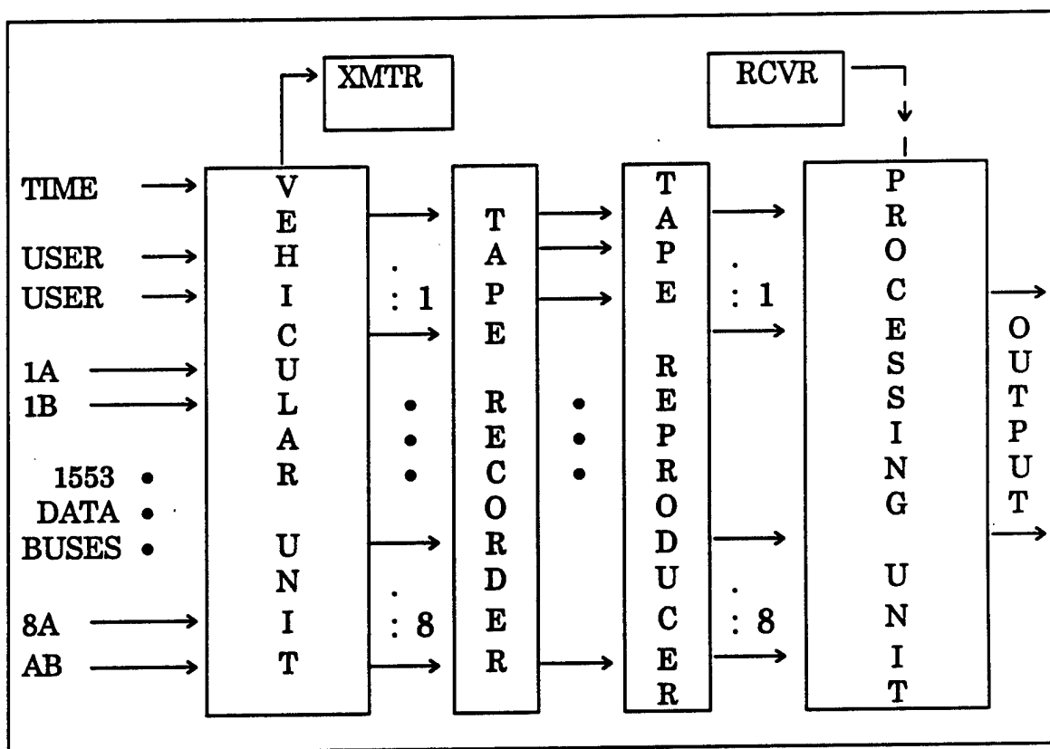
Figure 8-1. System block diagram.
