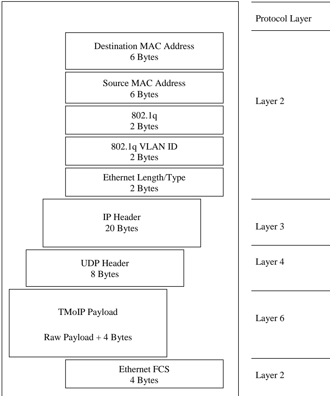
Figure 3-8. TMoIP Packet layout.
