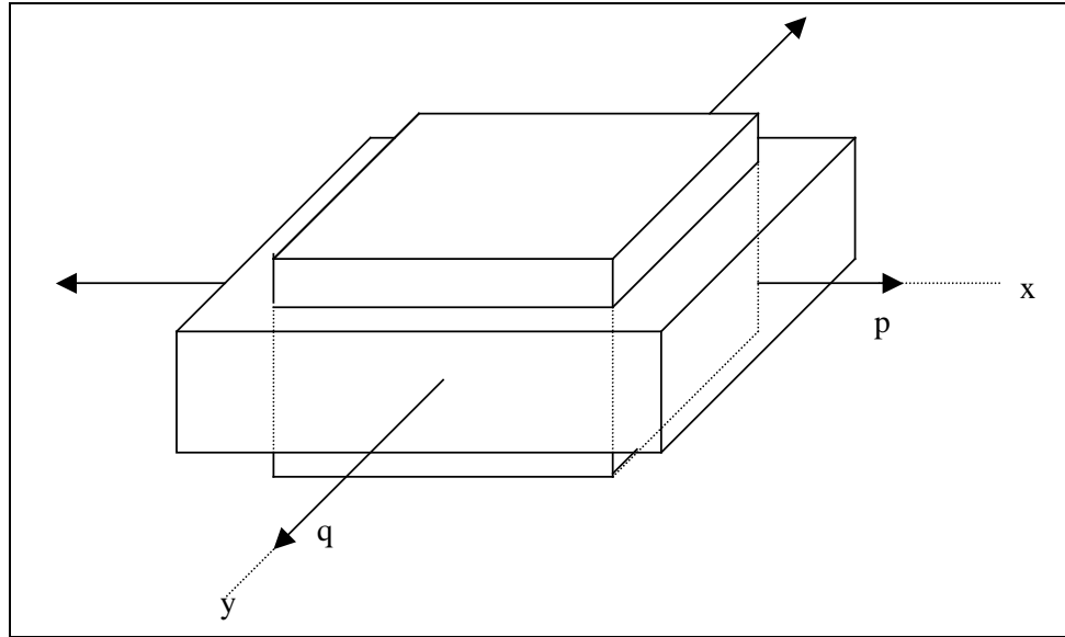
Figure 3-7. Bi-Axial Strain
