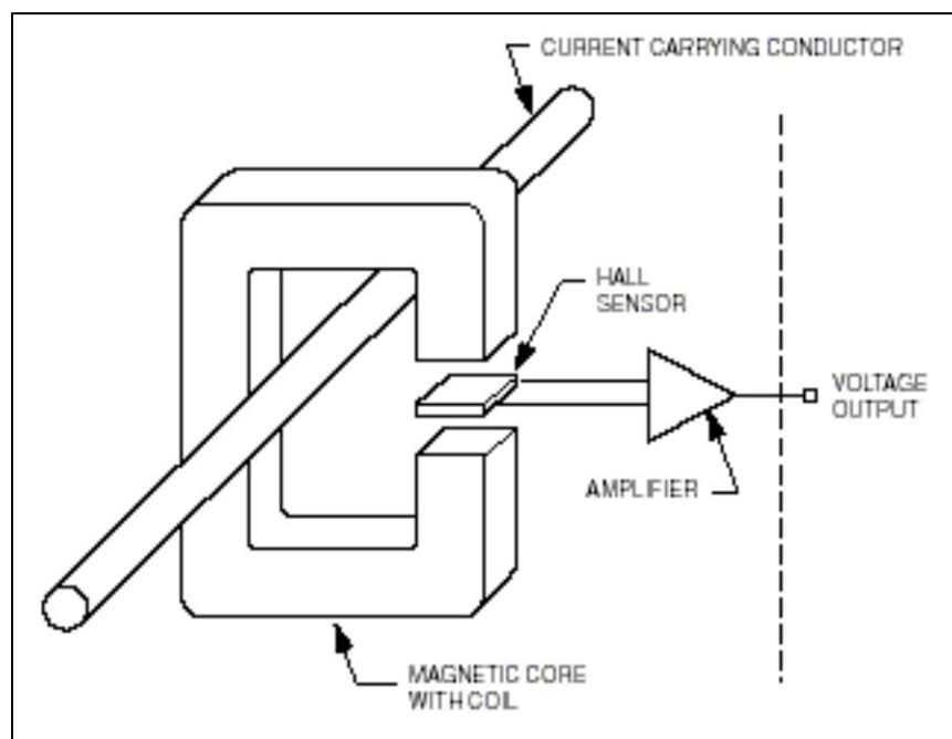
Figure 3-43. Hall Effect Current Transducer (Open Loop)
