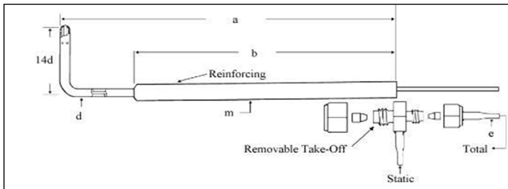
Figure 3-56. Type PD Probe
