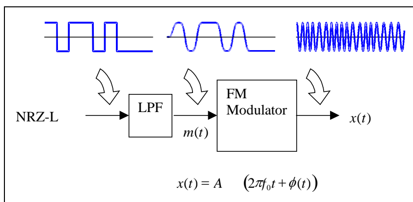
Figure 8-4. FM Modulator
