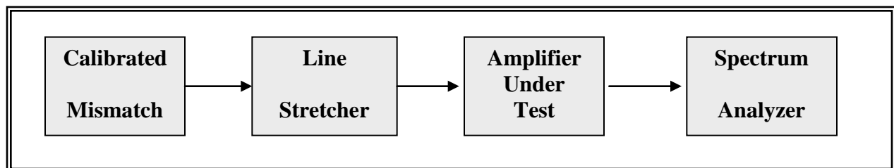
Figure 2-11. Impedance mismatch test setup (see test 2.6).
