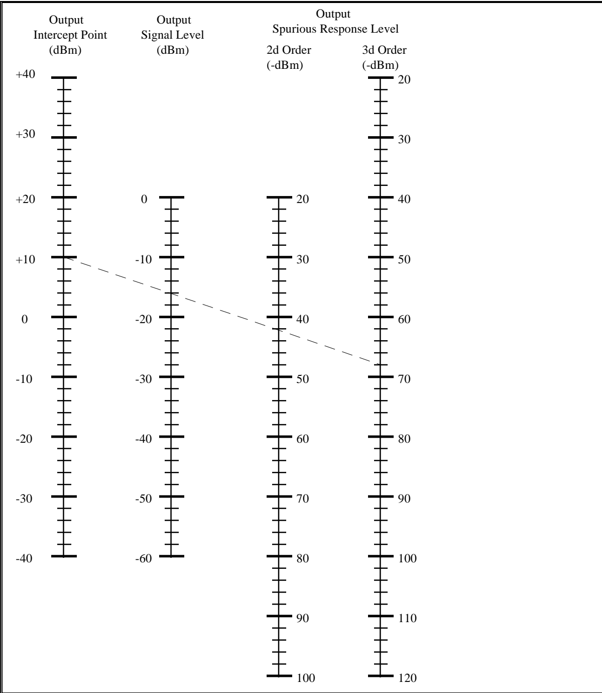
Figure 3-8. Spurious response nomograph (see test 3.3).
