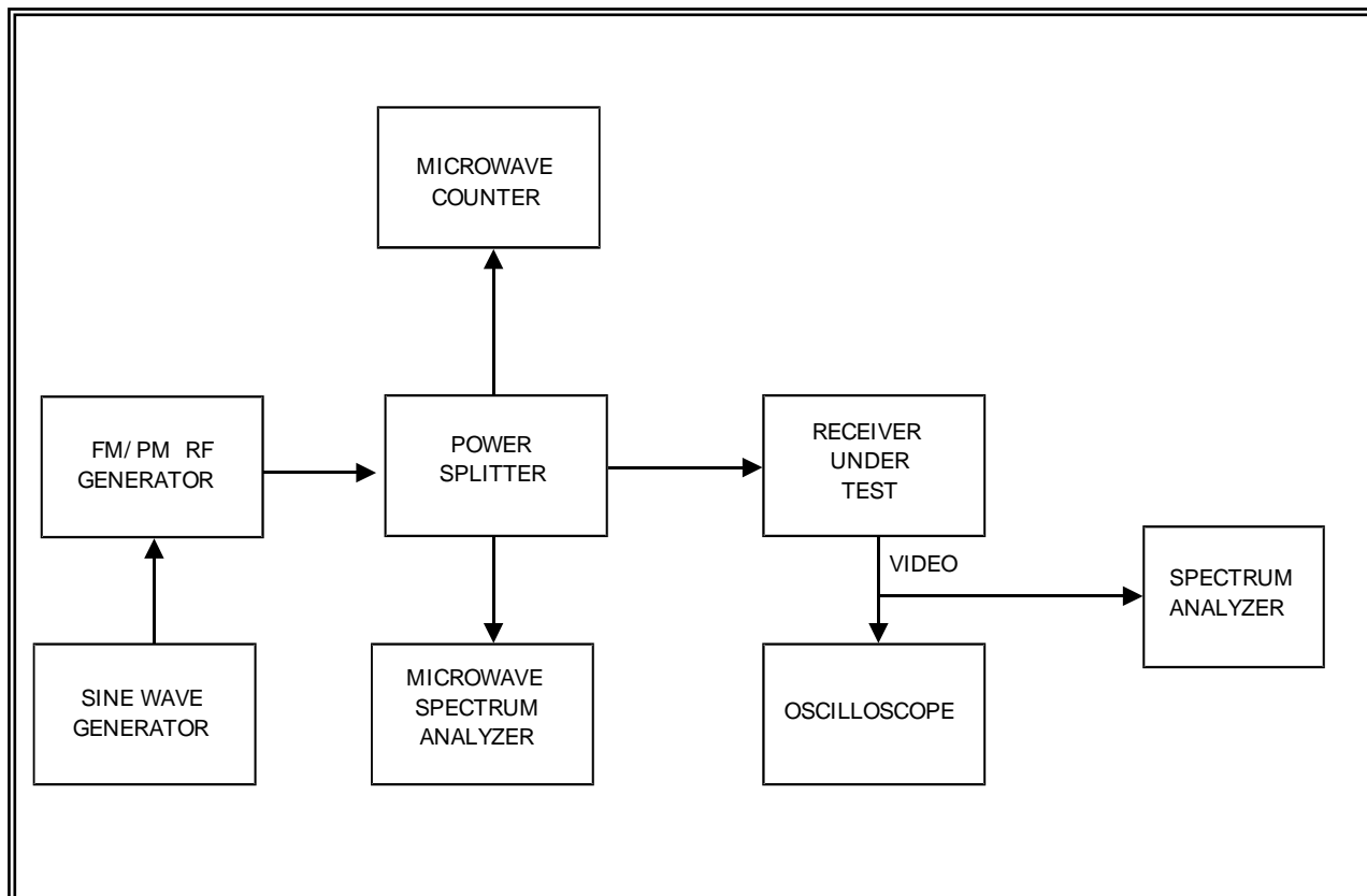
Figure 4-20. Receiver video spurious outputs (see test 4.18)
