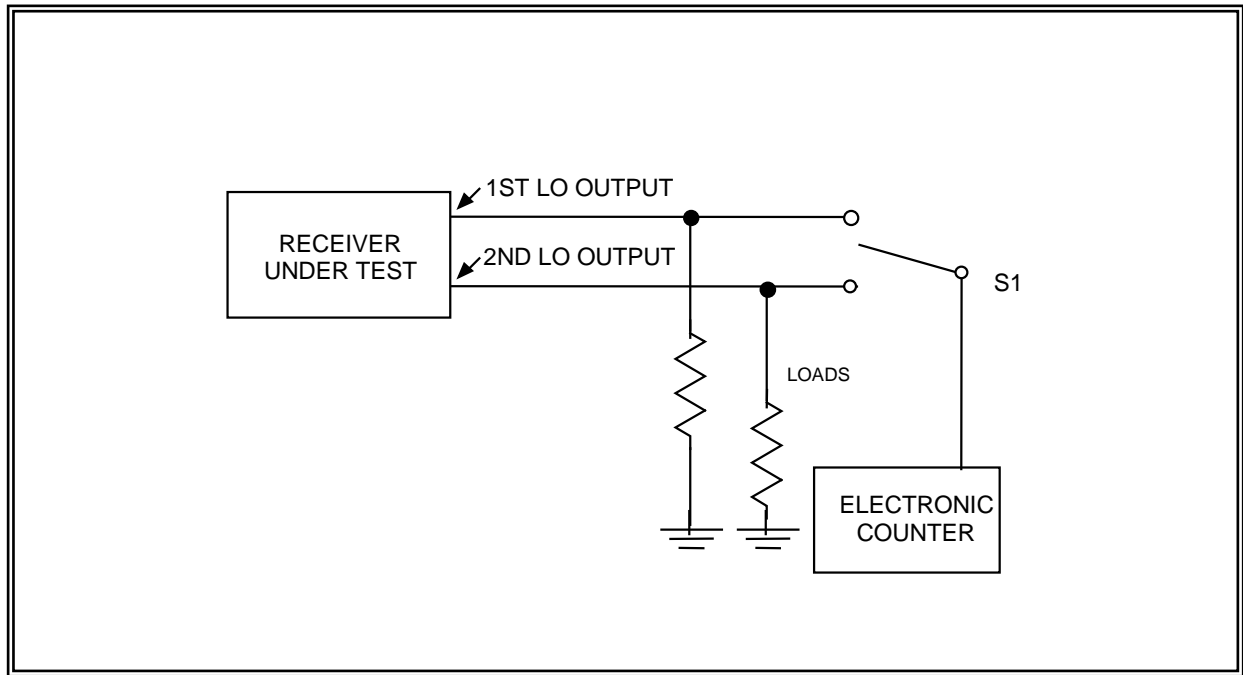
Figure 4-12. Local oscillator stability test (see test 4.10).
