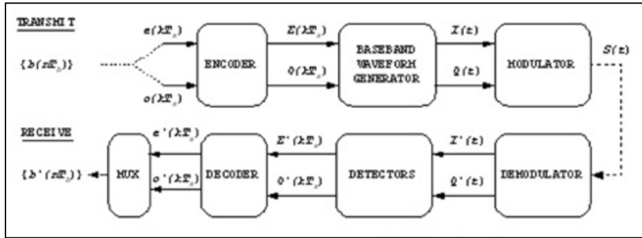
Figure M-1. Transmission System
