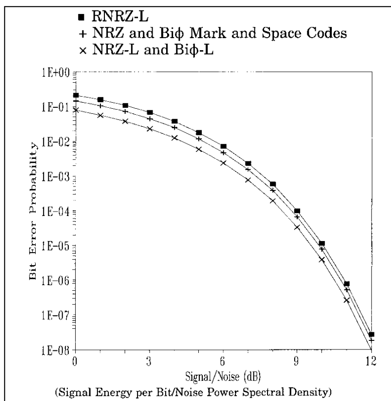
Figure C-3. Theoretical BEP Performance for Various Baseband PCM Signaling Techniques (Perfect Bit Synchronization Assumed)
