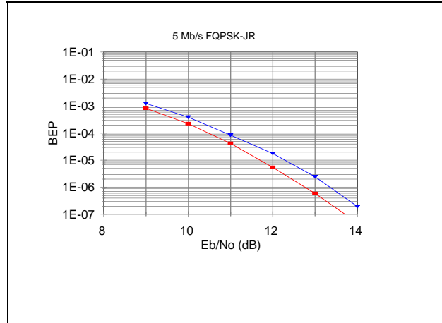
Figure A-21. FQPSK-JR BER vs. E_b/N_0 .
